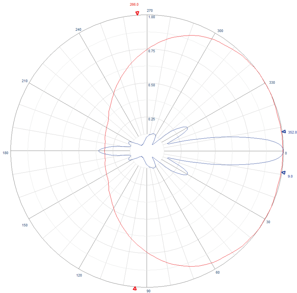
Example radiation pattern - Z4UD-520650
